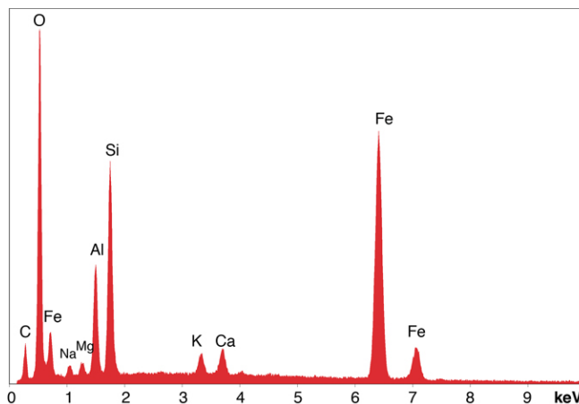
Fig. (24). Spheres formed during ignition of commercial thermite, with corresponding typical XEDS spectrum.
